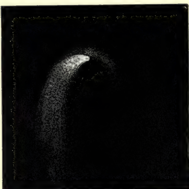
July 1.
